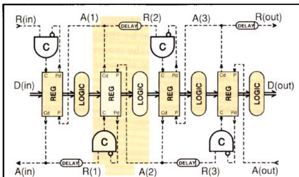
FIGURE 17. Micropipeline with Processing
