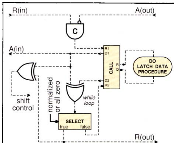
FIGURE 23. Control Circuit for a Sequential Normalizer
