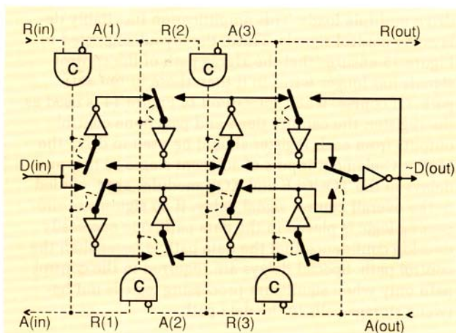
FIGURE 16. A FIFO Circuit
