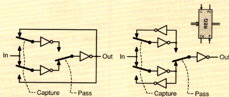
FIGURE 12. Event-Controlled Storage Elements
