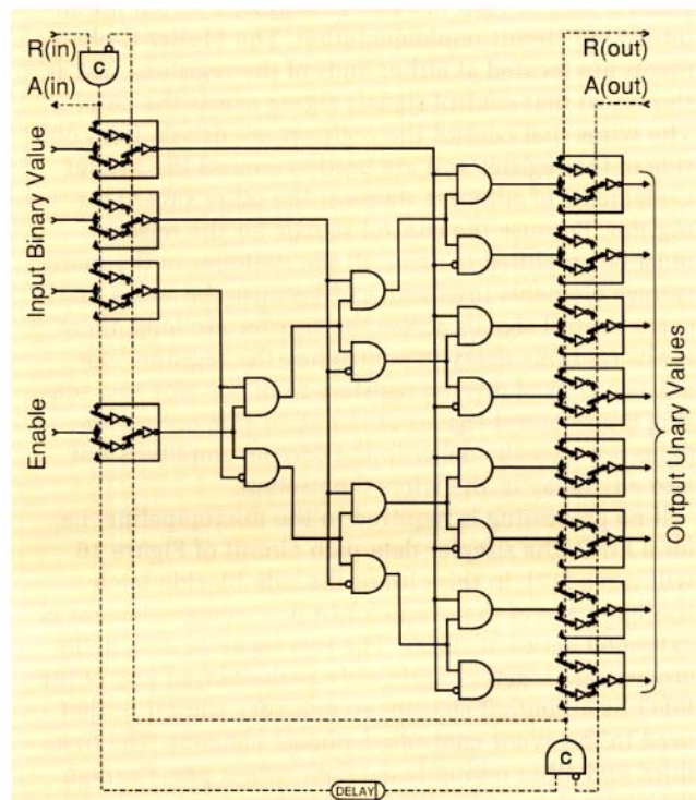
FIGURE 18. A Decoder with Two Micropipeline Stages
