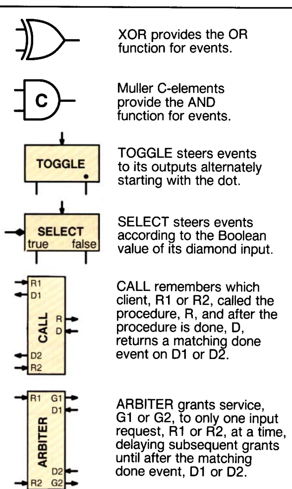
FIGURE 9. Logic Modules for Events
