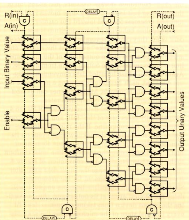
FIGURE 19. A Decoder with Four Micropipeline Stages
